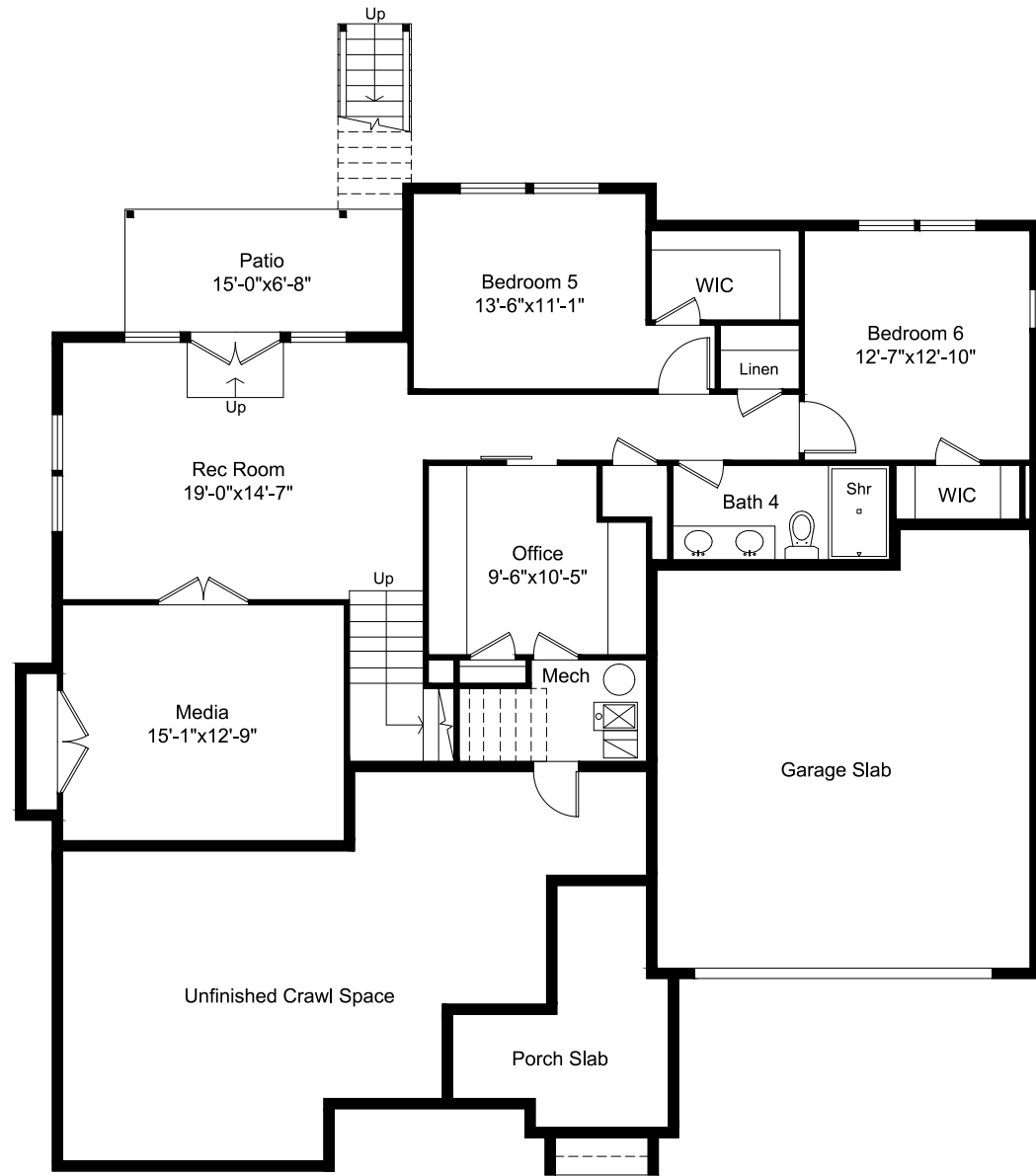
BASEMENT FLOOR
